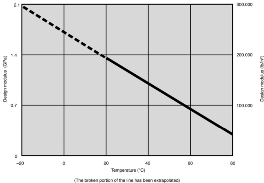
Figure 1 Design Modulus for Perspex® GS cast acrylic sheet as a function of temperature
