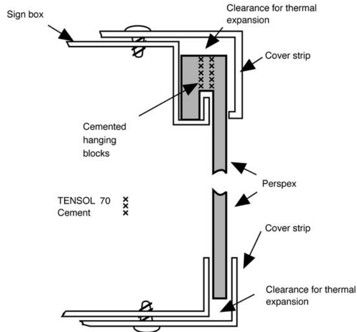
Figure 3 A typical design for top hanging bar
