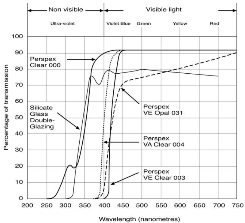
Figure 2 Spectral transmittance of 3 mm Perspex® from Lucite® GS cast sheet grades compared with silicate glass
