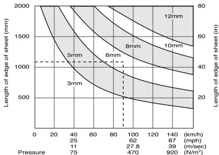
Figure 4 The recommended thicknesses of Perspex® for various wind loads when designing for rectangular windows, with all edges fully supported
